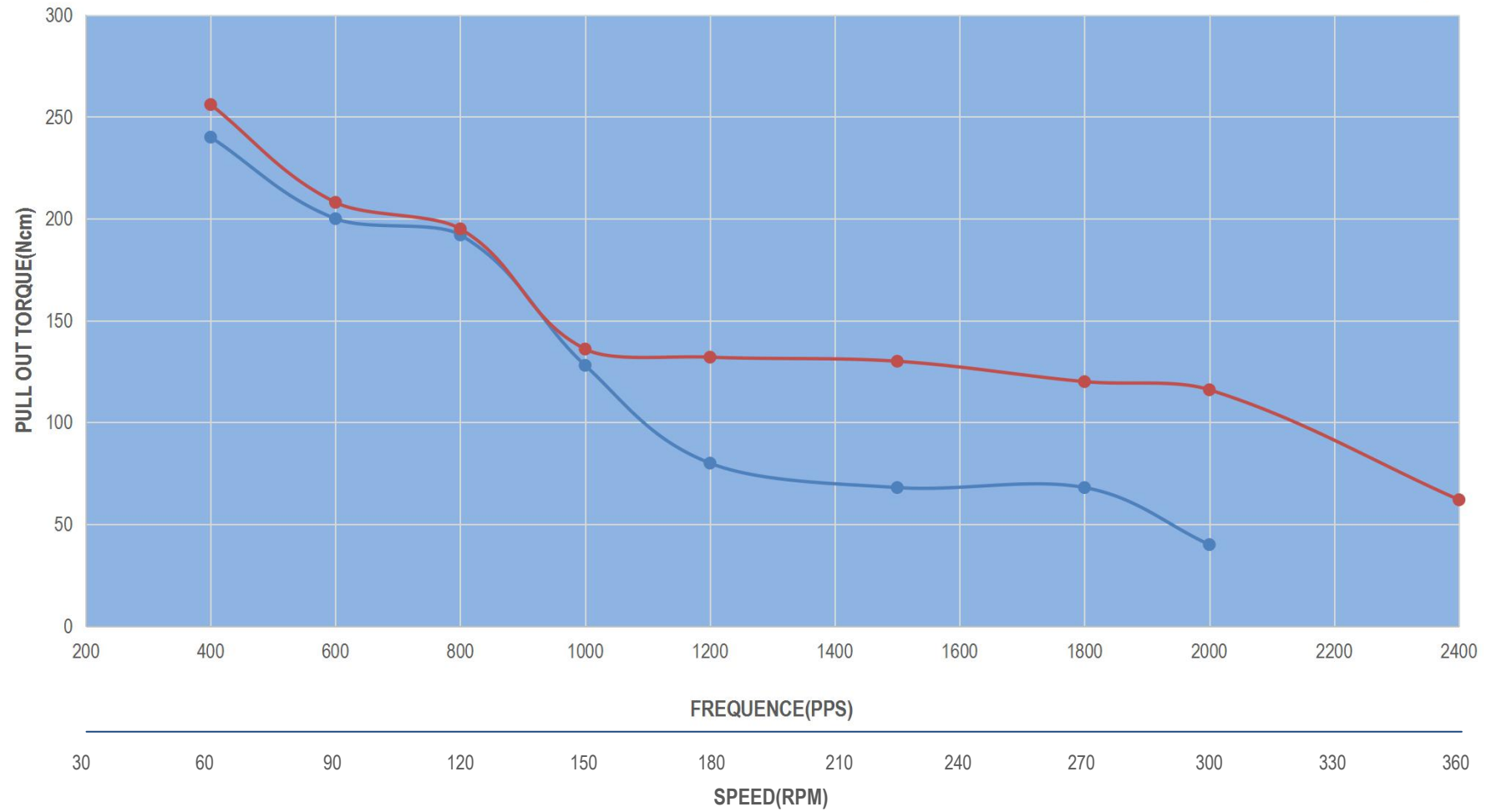
24HS34-3504D PULL OUT TORQUE(3.5A/P 24V/48V HALF STEP)
