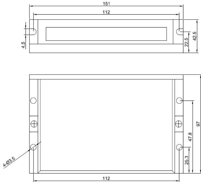
Figure 1: Mechanical specifications
