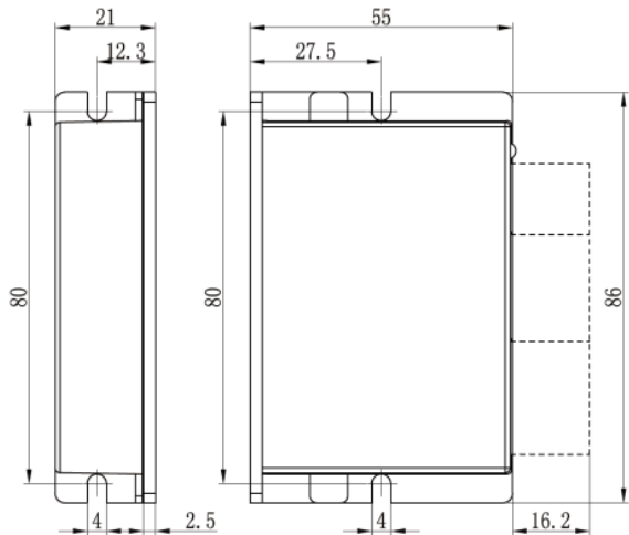
Figure 1: Mechanical specifications Recommend use side mounting for better heat dissipation
