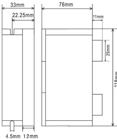
Figure 2: Mechanical specifications Recommend use side mounting for better heat dissipation
