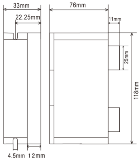
Figure 3: Mechanical specifications Recommend use side mounting for better heat dissipation
