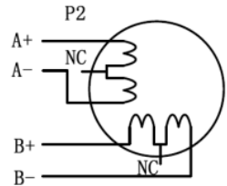
Figure 11: 6-lead motor full coil (higher torque) connections
