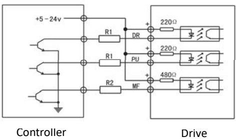
Figure 6: Independent common anode wiring method
