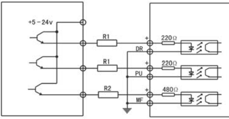
Figure 6: Independent common anode wiring method
