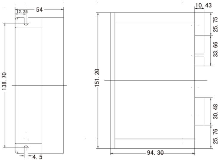
Figure4: Mechanical specifications Recommend use side mounting for better heat dissipation
