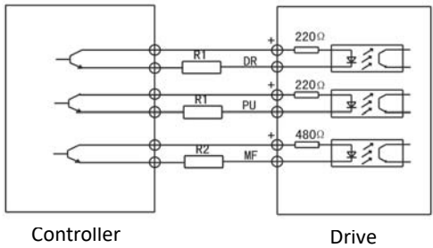
Figure 5: Differential wiring method
